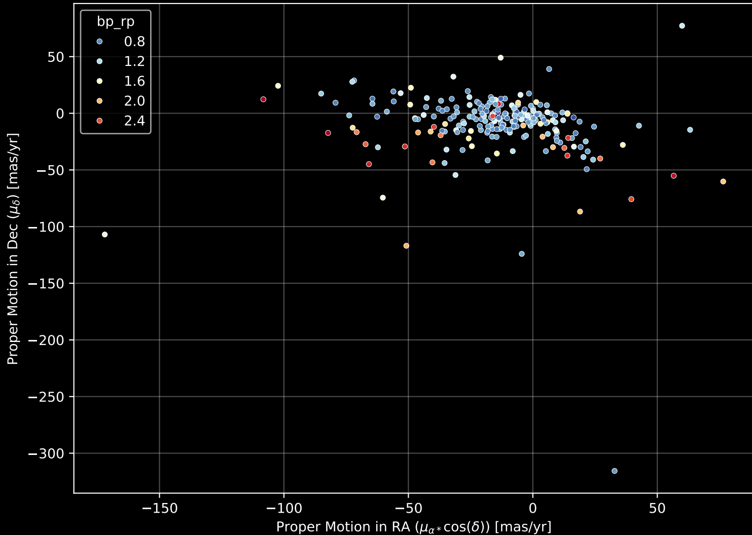
APOGEE DR17 Field: [266+65-O] Proper Motion Diagram (n= 232)
