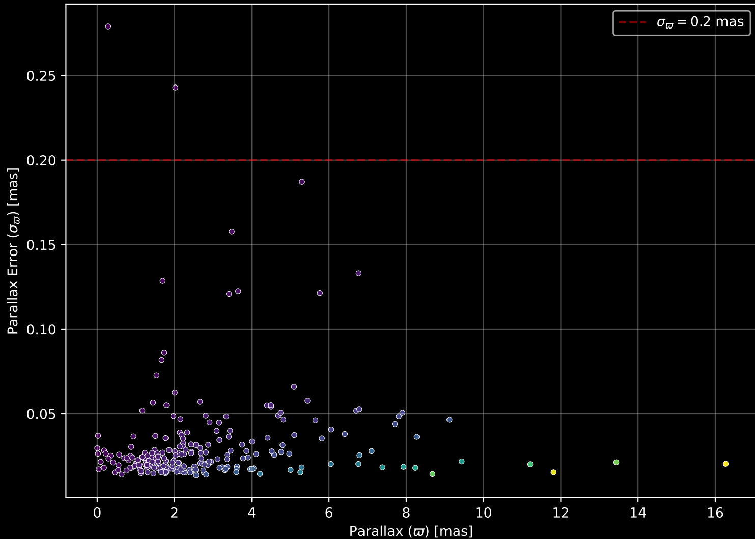
APOGEE DR17 Field: [266+65-O] Parallax Quality (n= 232)
