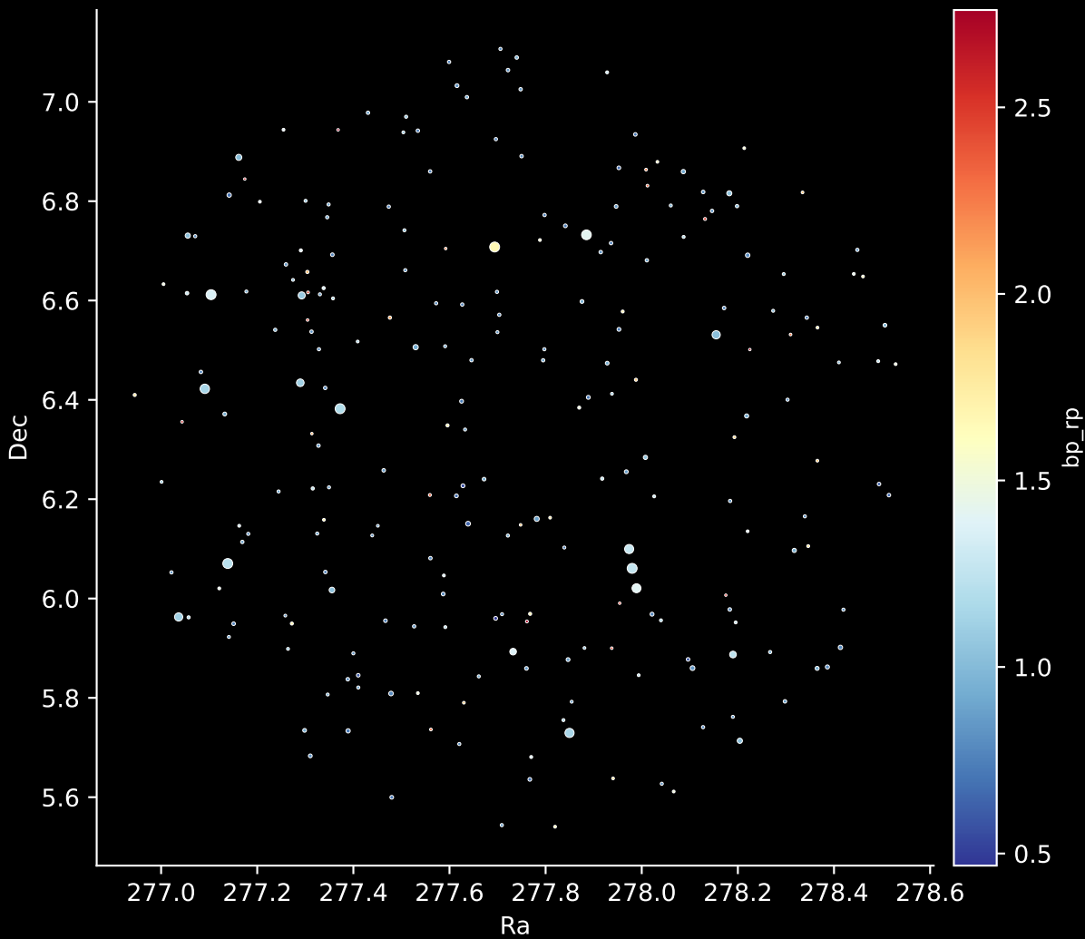
APOGEE DR17 Field: [266+65-O] Stars: 232
