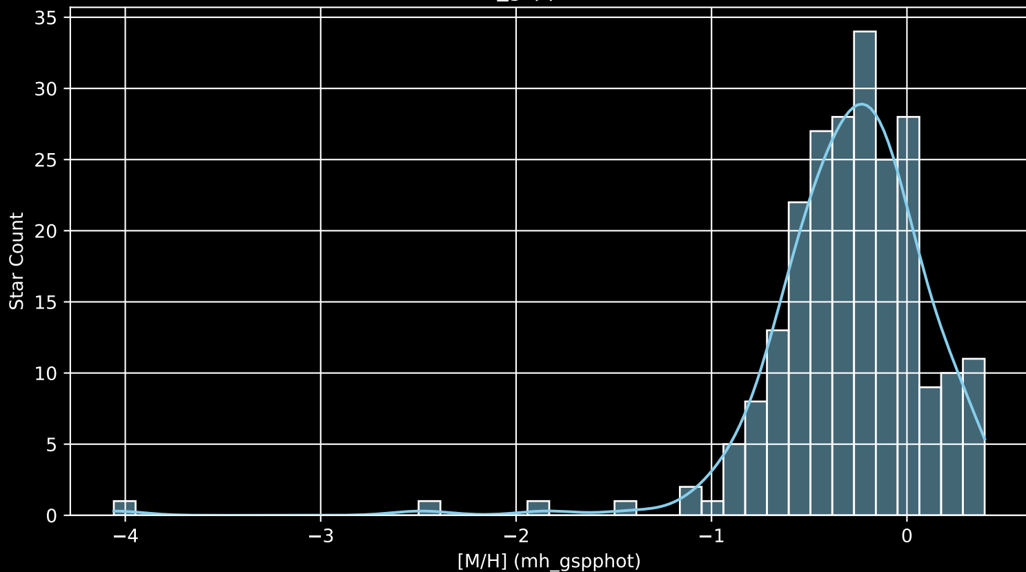
APOGEE DR17 Field: [266+65-O [M/H] (mh_gspphot) (n= 227)
