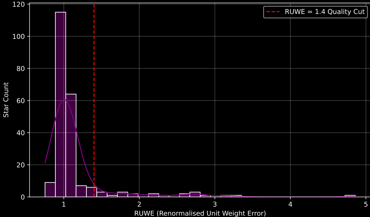
GAPOGEE DR17 Field [266+65-O] RUWE Distribution (n= 222)
