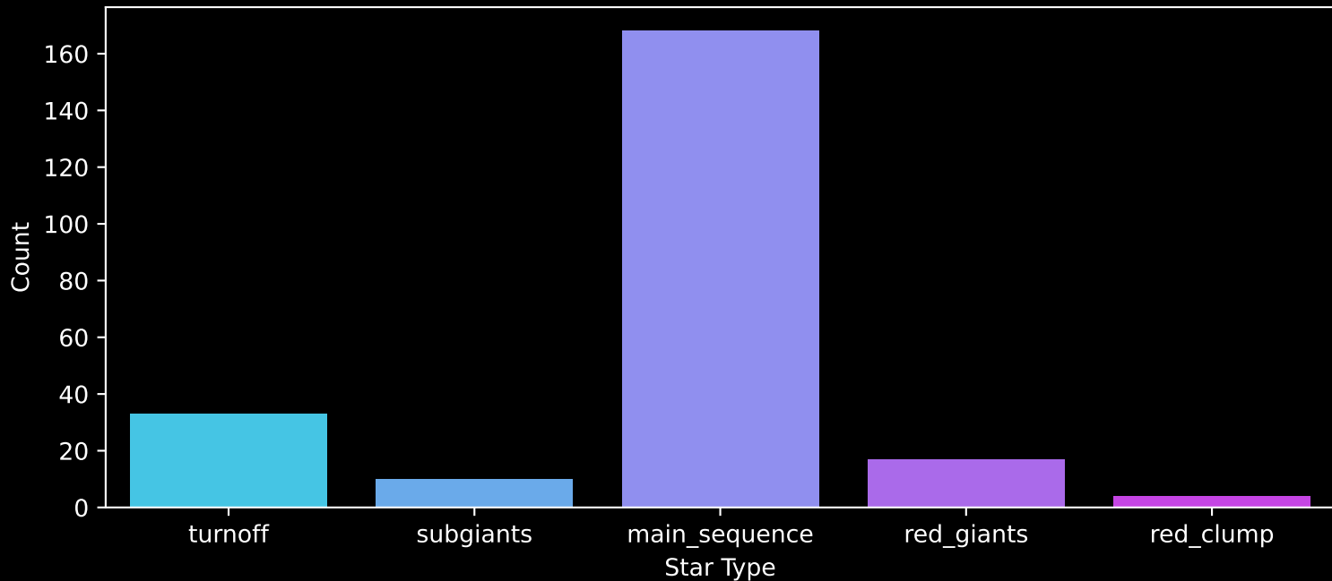
APOGEE DR17 Field: [266+65-O] Count plot of Star Type
